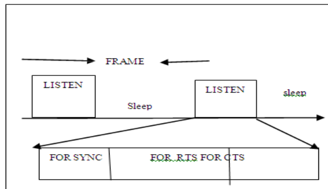
Fig. 1. Low Duty Cycle Operation of S-MAC [3]
